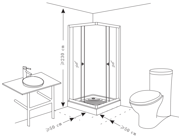
PLACE CHOOSING FOR MOUNTING
